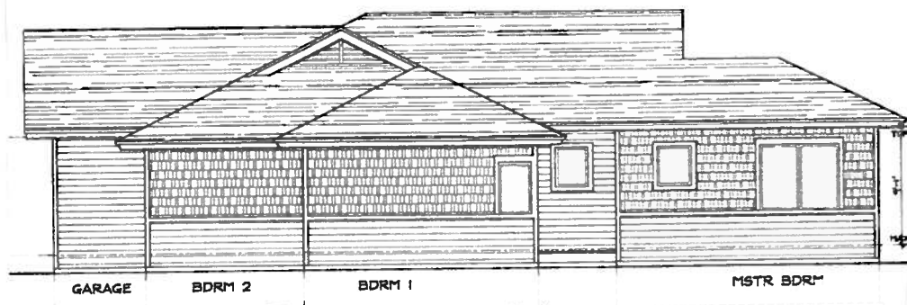
WEST ELEVATION 1/4" SCALE
