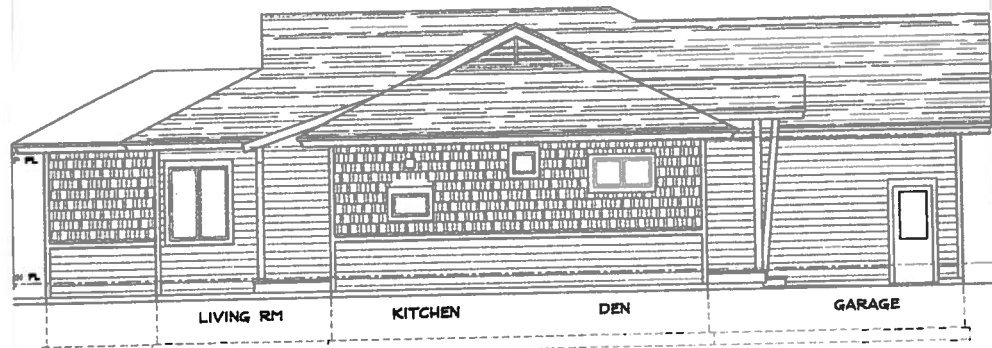
EAST ELEVATION 1/4" SCALE
