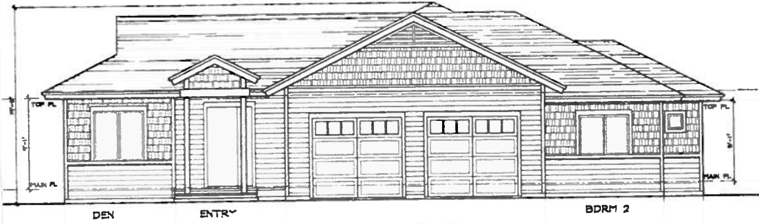
NORTH ELEVATION 1/4" SCALE
