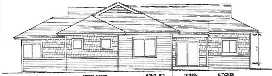
SOUTH ELEVATION 1/4" SCALE
